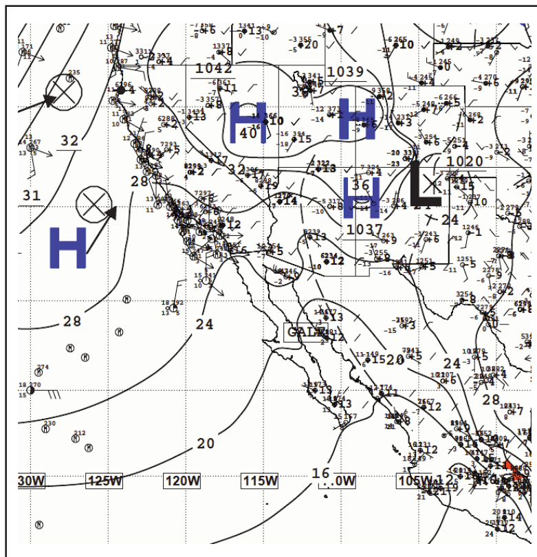
Figure 1. National Weather Service Unified Surface Analysis (USA) Valid 0600 UTC 05 February 2016
