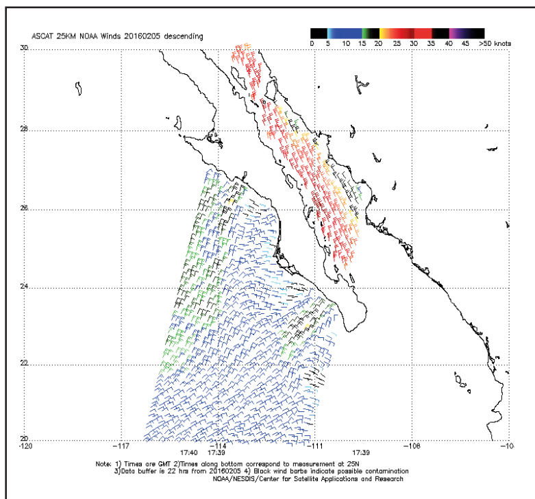
Figure 2. European Advanced Scatterometer (ASCAT) Pass Valid at 1739 UTC 05 February 2016
